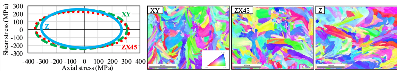
Figure 1. Initial yield surfaces at 10µε offset definition of yield and IPF maps of three printing orientations.
